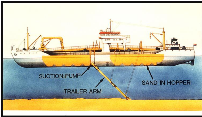
Govva 29: Typihkalaš hopper- čiekŋudeaddji njámmannrusttegiinnis (trailing suction hopper dredger).
