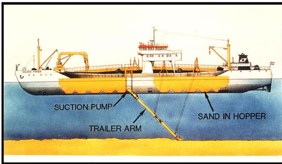
Govva 51: Typihkalaš hopper-čiekŋudeaddji ovtta njammanrusttegiinnis (trailing suction hopper dredger).
